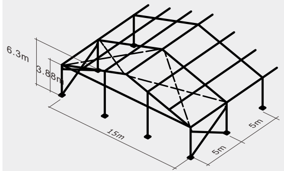
Type BT15/400
