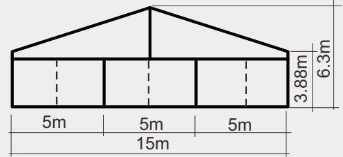
Type BT15/400
