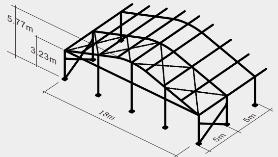
Type DET18/330
