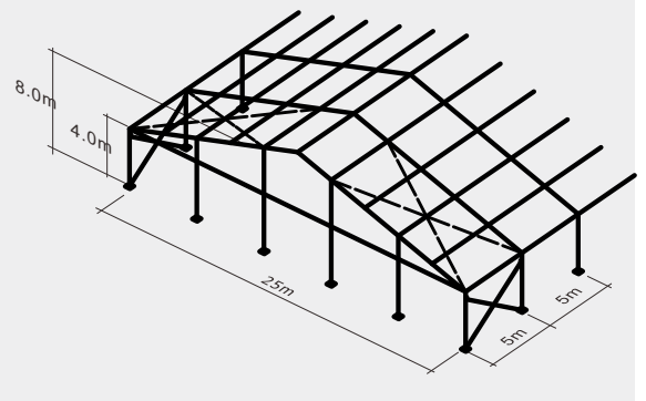
Type EBT25/400
