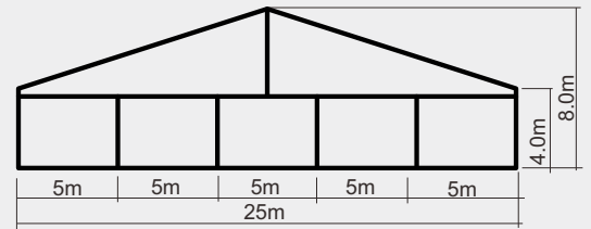
Type EBT25/400
