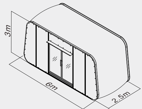
(Type: MB-ETA6/300)
