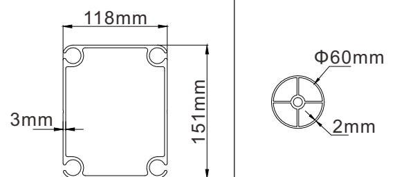
Main frame
