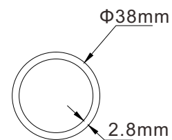
Eave beam
