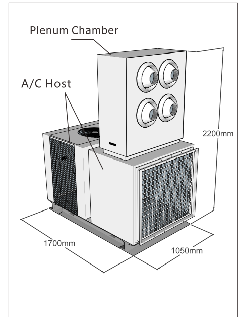
Perspective View
