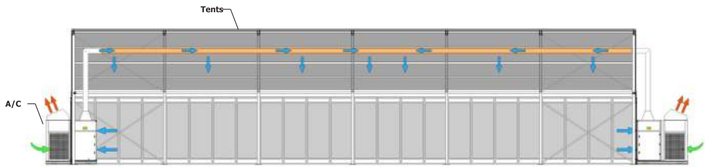
Demonstration of A/C Installed Inside and Outside the Tent Gable Side
